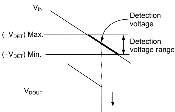
Figure 29 Detection Voltage
