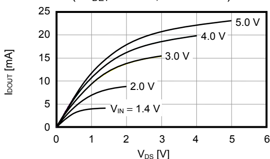
S-1701xxx55 ( -V_{DET} = 5.5\text{ V} , T_a = 25\text{ °C} )
