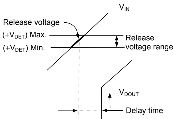
Figure 30 Release Voltage
