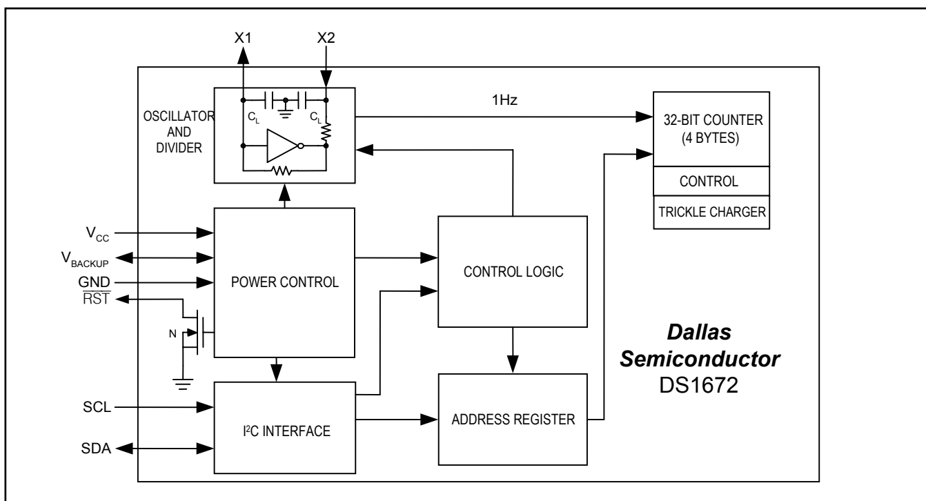
Figure 4. Block Diagram
