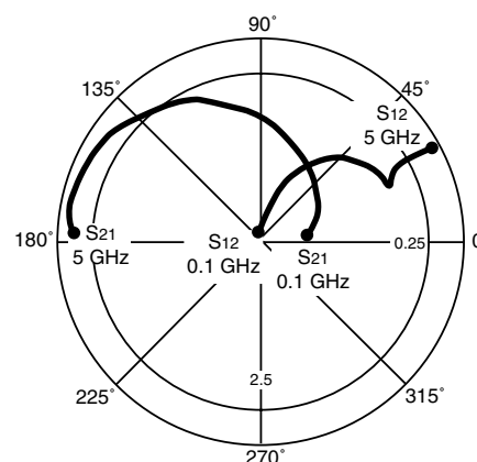
Coordinates in Ohms Frequency in GHz ( V_{CE} = 1\text{ V} , I_C = 1\text{ mA} )
