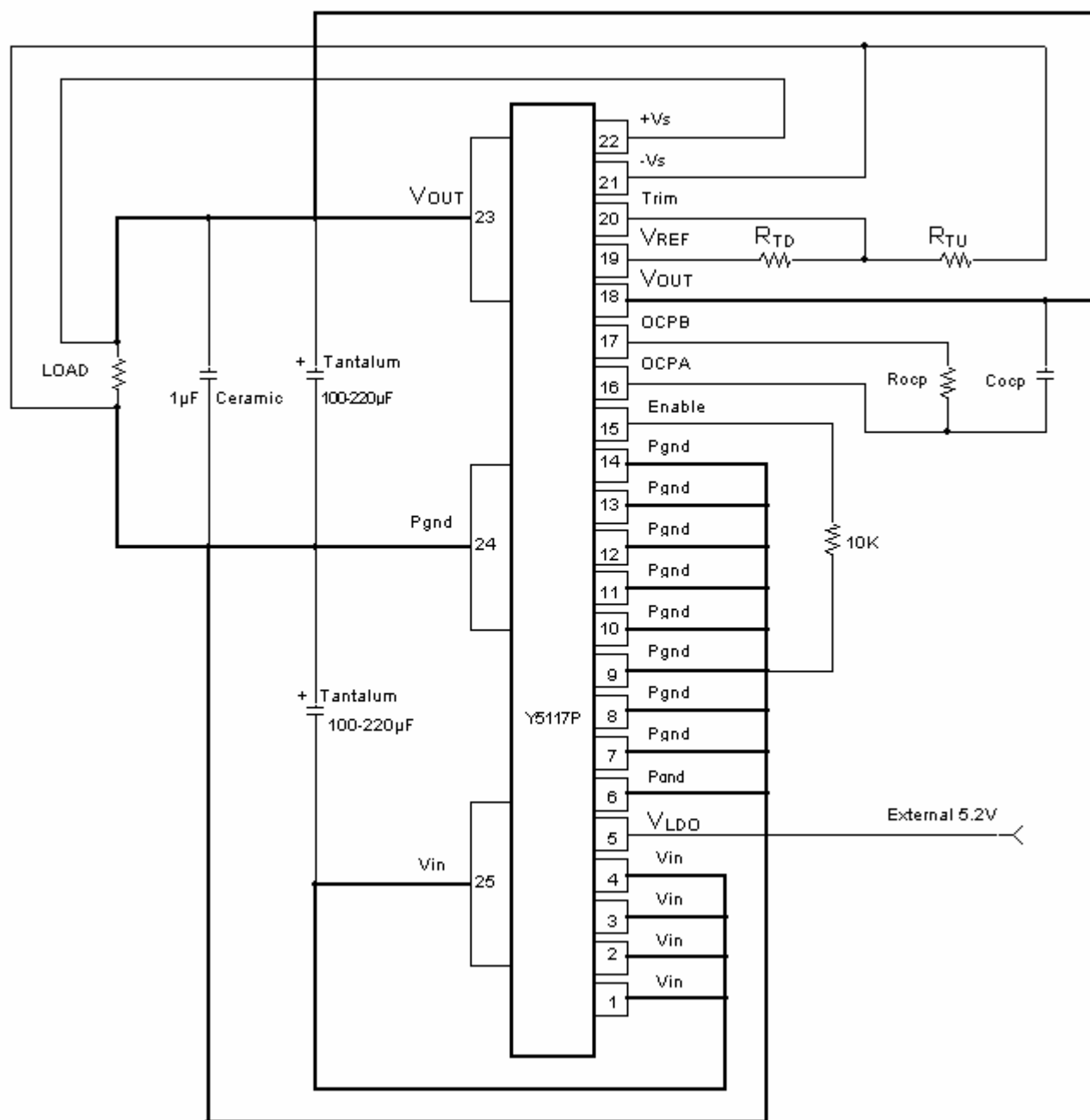
Figure 12. Typical Application Circuit for 5.2VDC > V_{in} ≥ 3.0VDC. V_{LD0} is connected to the external voltage source. 10kΩ resistor is placed between the Enable pin and Pgnd .
