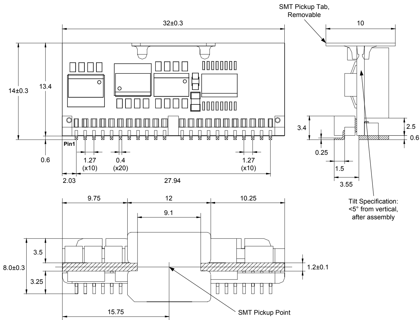
Figure 13. Mechanical Drawing
