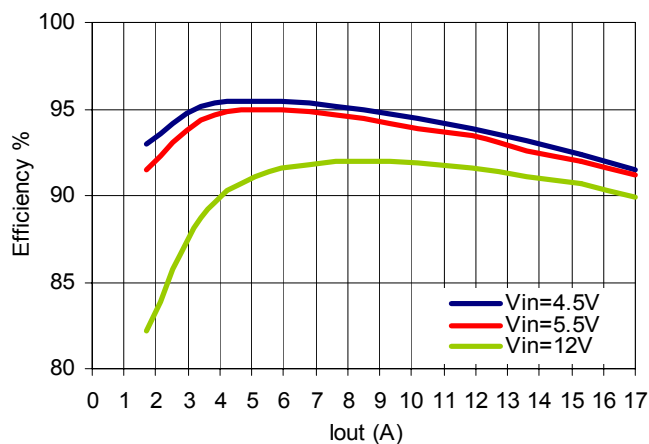
Figure 3. Efficiency Vs. Load at Vout=3.3V
