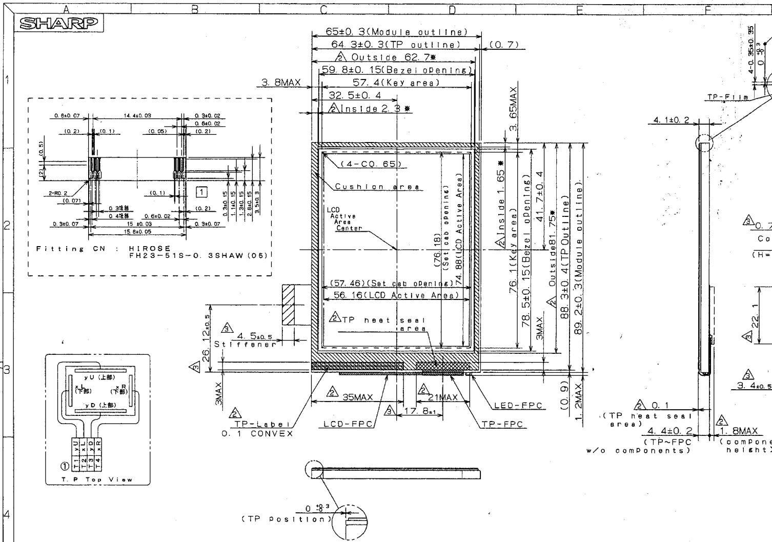
Fig. 1 Outline dimensions
