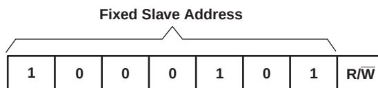
Figure 5. TCA6507 Address
