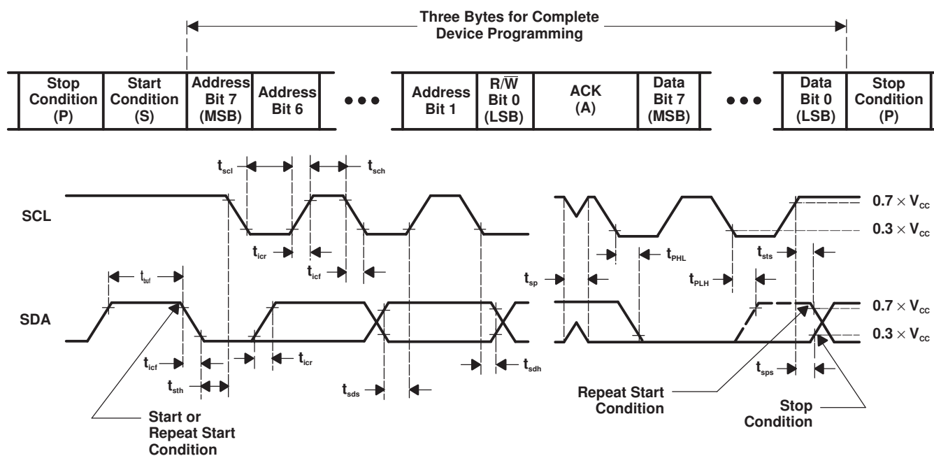
VOLTAGE WAVEFORMS
