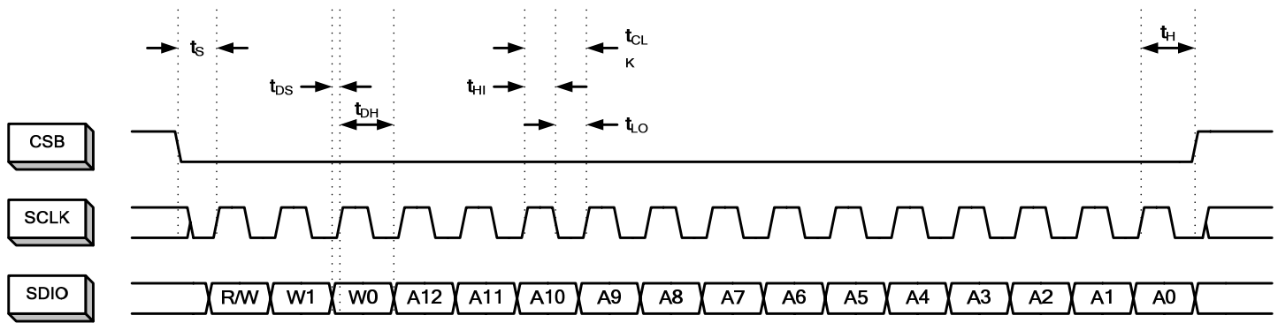
Figure 42. Instruction/Address Phase
