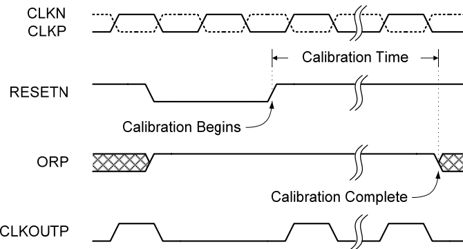
Figure 29. Calibration Timing
