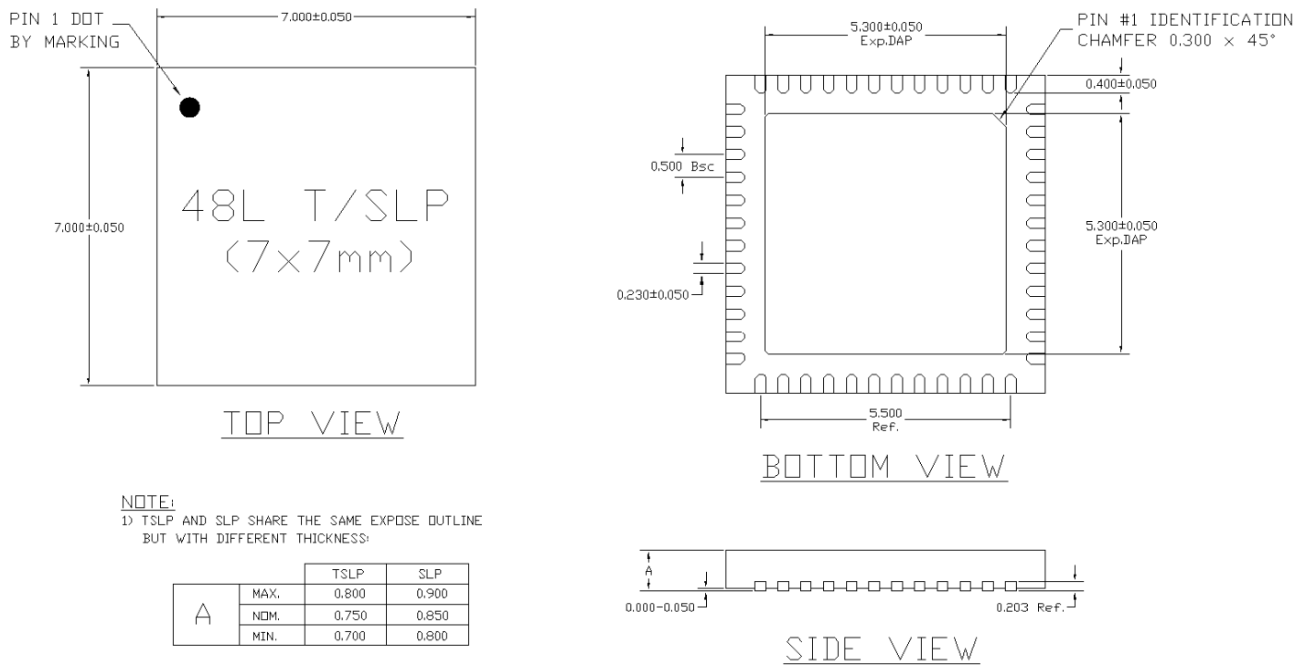
Figure 55. 48QFN Dimensions
