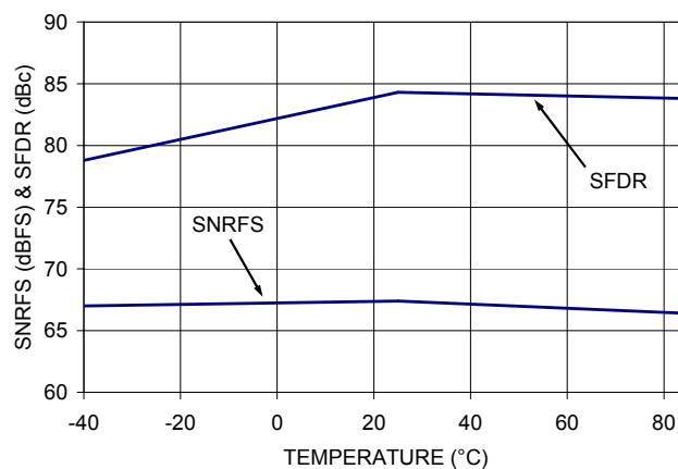
Figure 26. SNR & SFDR vs. Temperature
