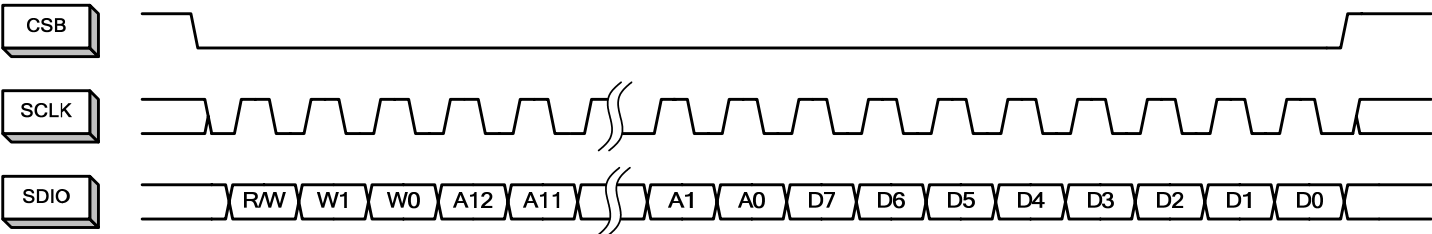
Figure 40. MSB-First Addressing
