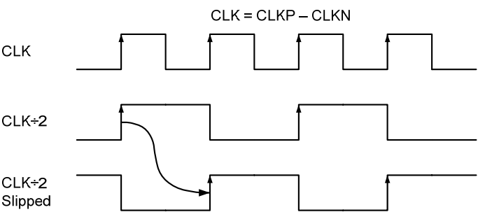
Figure 45. Phase Slip
