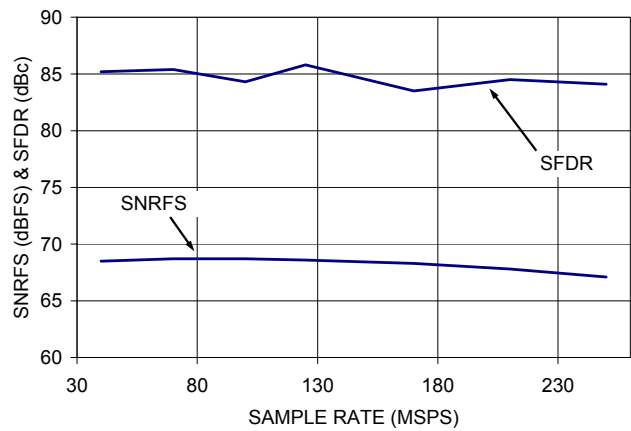
Figure 9. SNR & SFDR vs. f_{SAMPLE}
