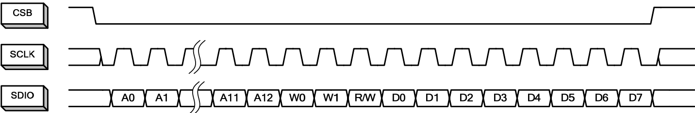
Figure 41. LSB-First Addressing
