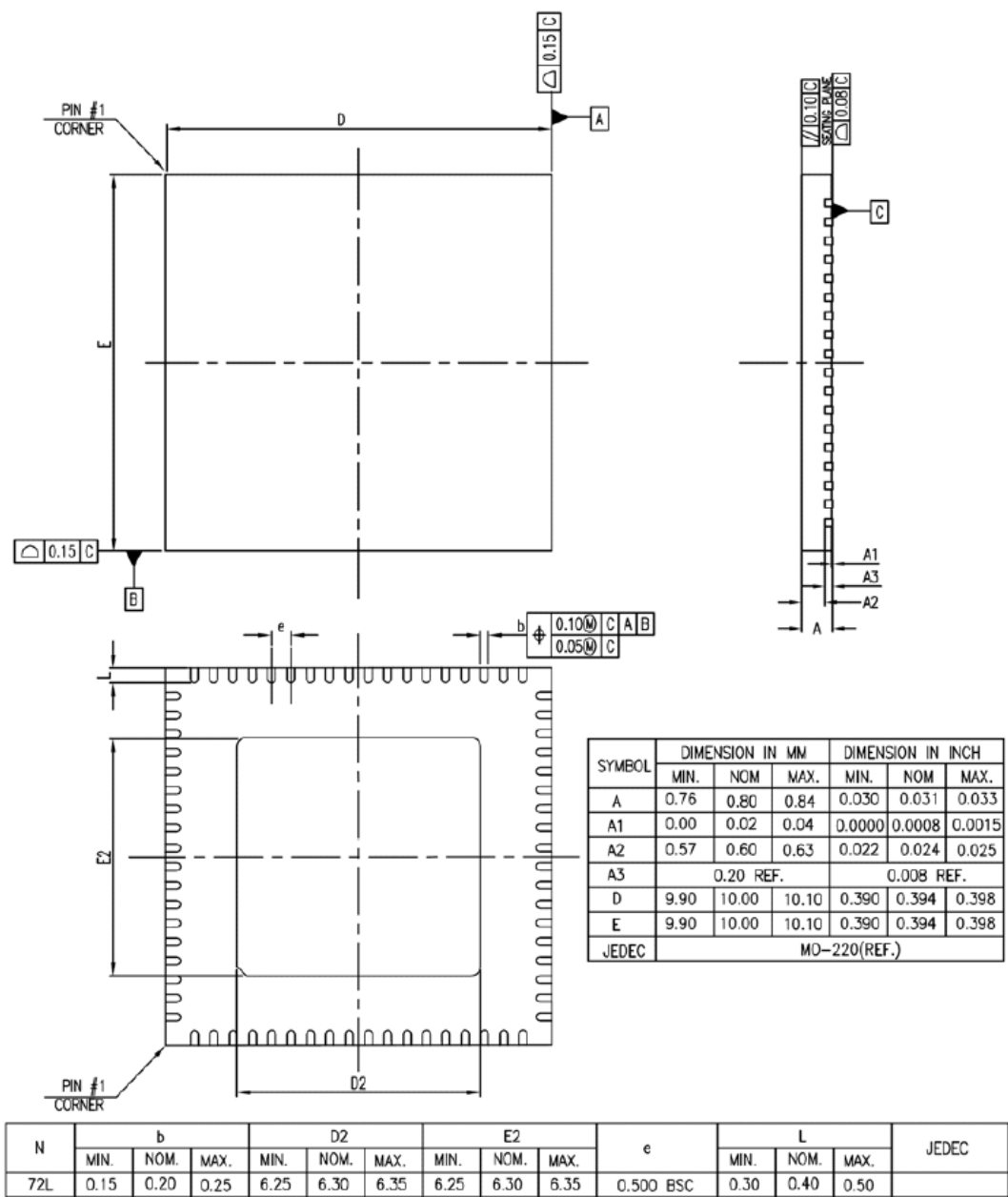
Figure 54. 72QFN Dimensions
