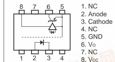
PIN CONNECTIONS (Top View)
