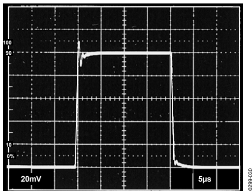
Figure 30. Small Signal Transient Response ( C_{LOAD} = 100 \text{ pF} , A_{VCL} = 1 )
