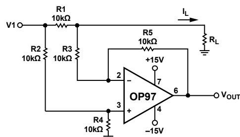
Figure 36. Current Monitor
