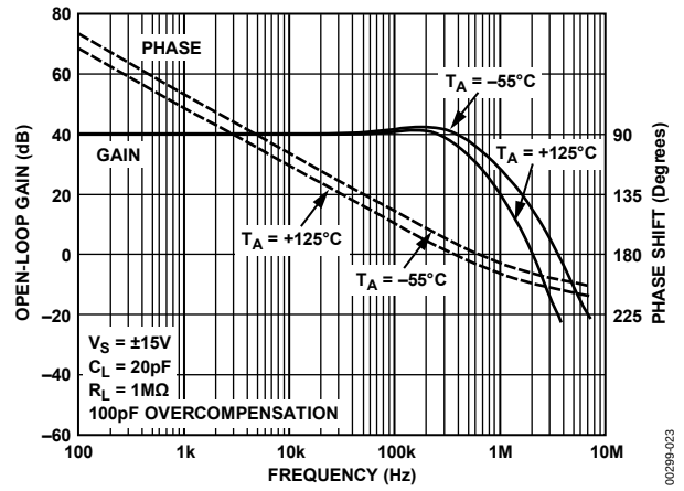
Figure 23. Open-Loop Gain, Phase vs. Frequency ( C_{OC} = 100 \text{ pF} )
