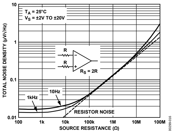
Figure 16. Total Noise Density vs. Source Resistance
