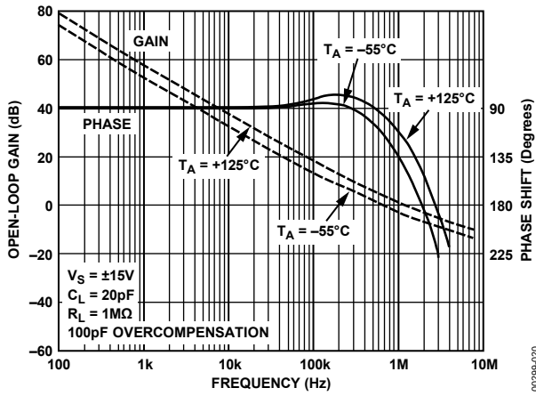
Figure 20. Open-Loop Gain, Phase vs. Frequency ( C_{OC} = 0 \text{ pF} )
