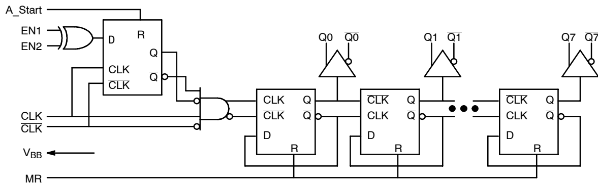
Figure 2. Logic Diagram
