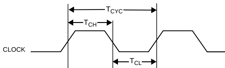
Figure 18. Clock Timing
