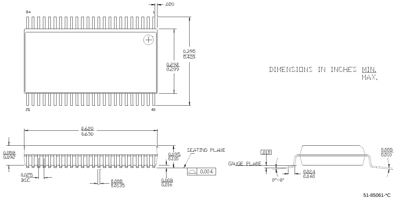
Figure 29. 48-Lead Shrunk Small Outline Package O48
