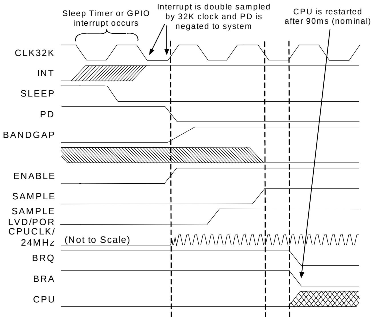
Figure 9. Wakeup Timing
