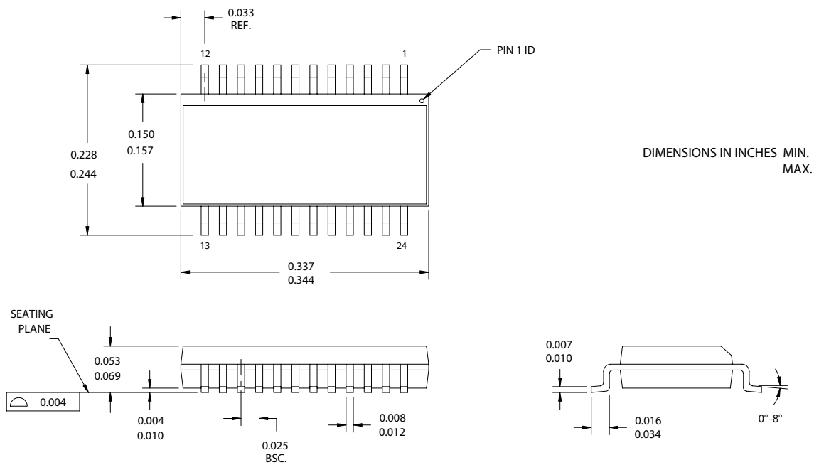
Figure 26. 24-lead QSOP O241
