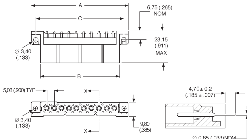
Section X-X
