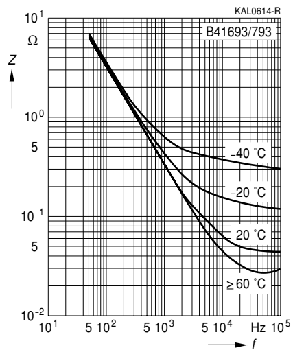
Impedance Z versus frequency f at different temperatures Typical behavior for 470 \mu\text{F}/63 \text{ V}
