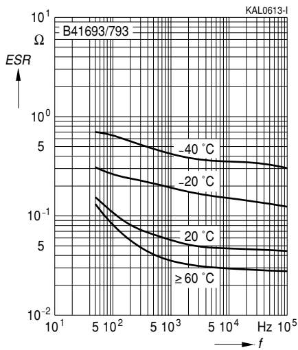
Equivalent series resistance ESR versus frequency f at different temperatures Typical behavior for 470 \mu\text{F}/63 \text{ V}
