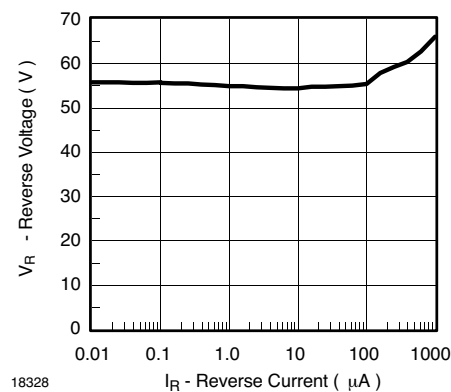
18328 Figure 4. Reverse Voltage vs. Reverse Current
