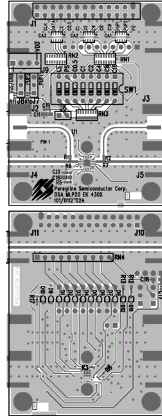
Figure 15. Evaluation Board Layout
