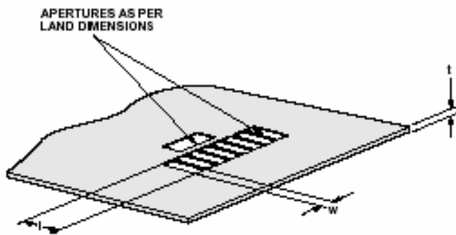
Figure A3. Solder stencil aperture
