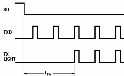
Figure 5e. Timing Waveform - TXD Wakeup Time Waveform
