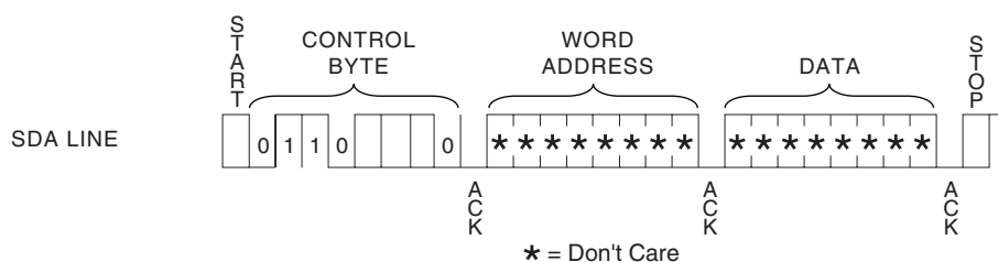
Figure 7. Setting Write Protect Register
