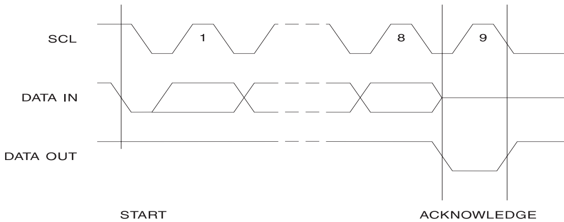
Figure 6. Output Acknowledge
