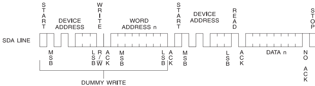
Figure 12. Random Read
