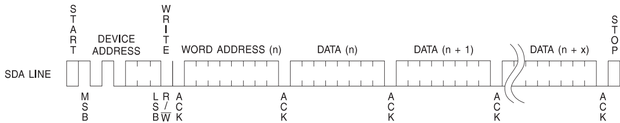
Figure 10. Page Write
