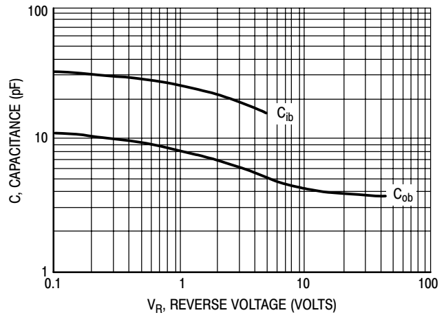
Figure 7. Capacitances
