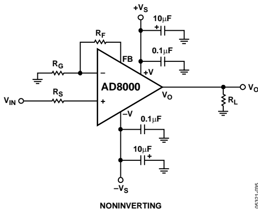
Figure 50. Noninverting Configuration
