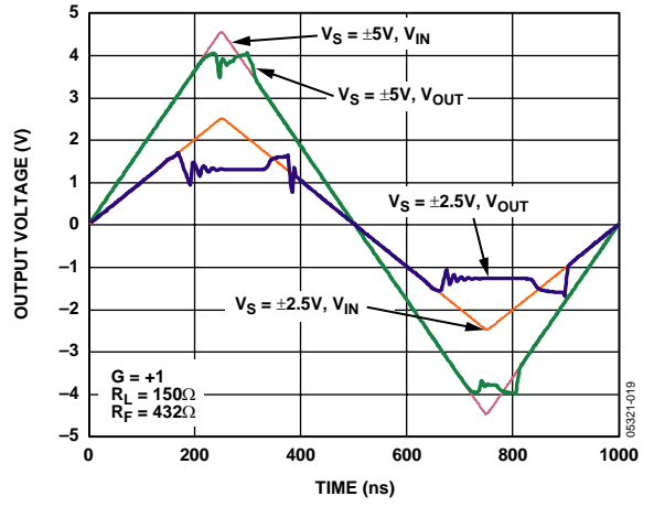
Figure 38. Input Overdrive
