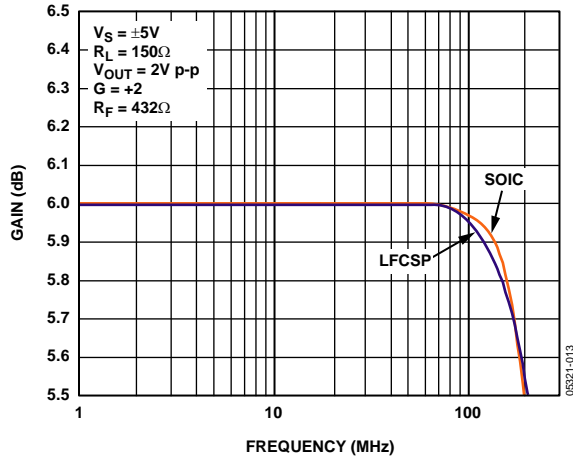
Figure 13. 0.1 dB Flatness
