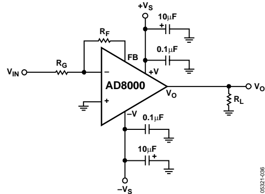
Figure 51. Inverting Configuration
