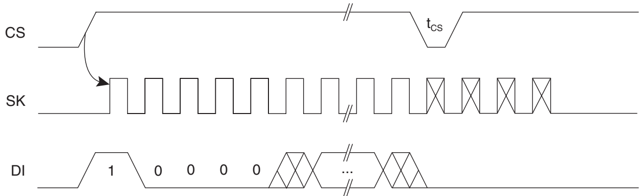
Figure 5. EWDS Timing
