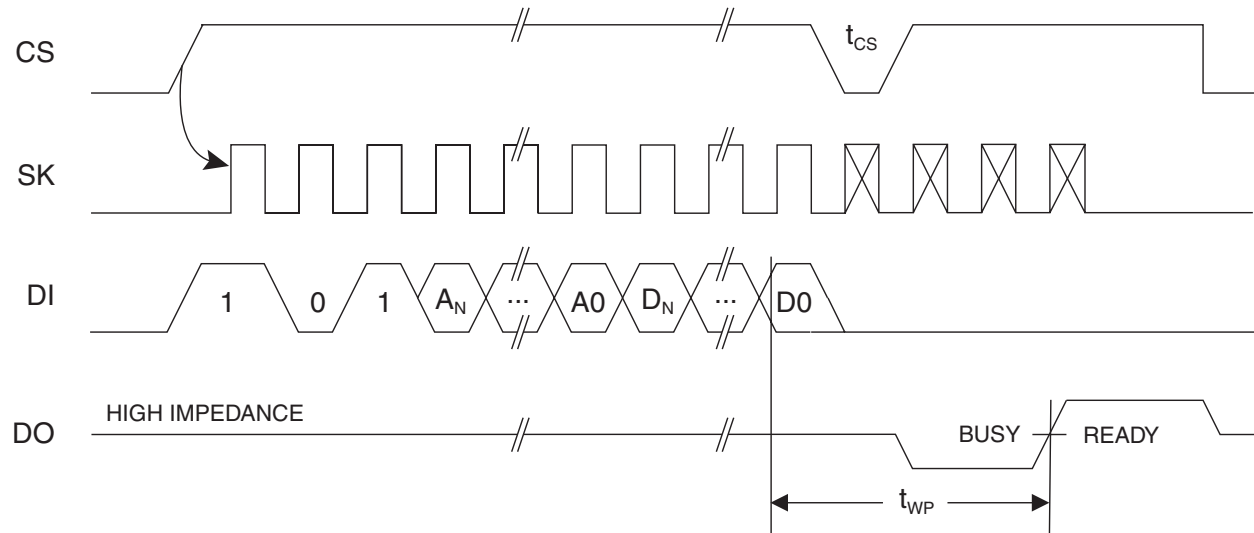
Figure 6. WRITE Timing
