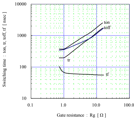
Switching time vs. Gate resistance (typ.) V_{cc}=600V, I_c=600A, V_{GE}=\pm 15V, T_j=25^\circ C
