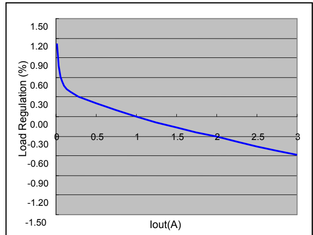
Load Regulation
