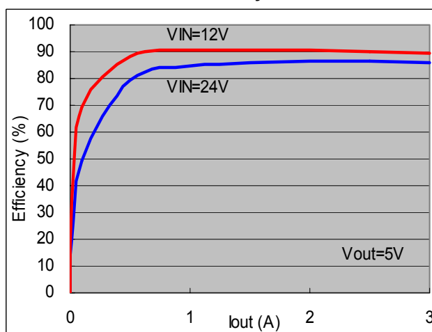
Efficiency
