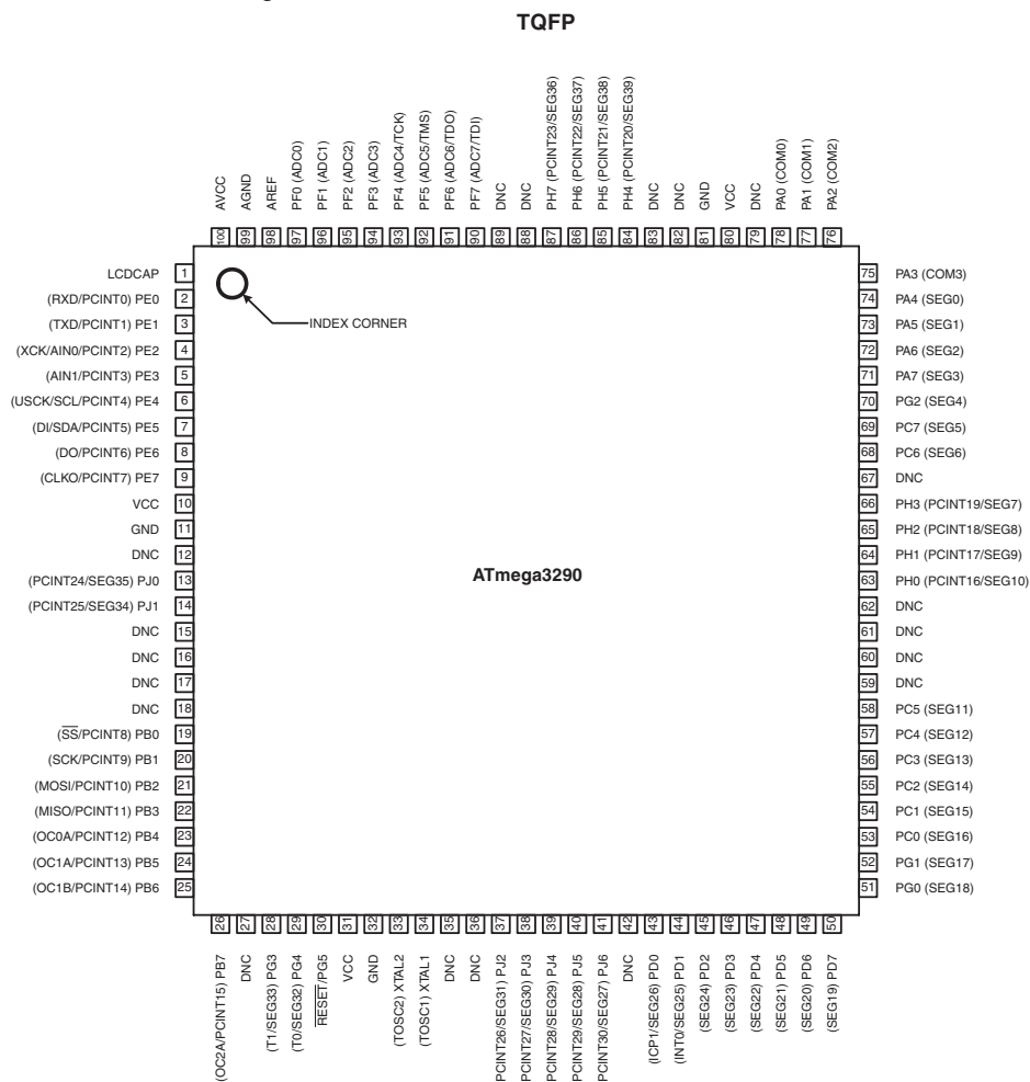
Figure 1-1. Pinout ATmega3290P
