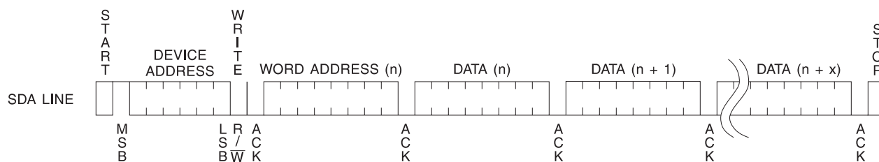
Figure 9. Page Write
