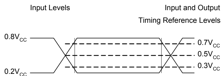
Figure 20. AC Measurement I/O Waveform
