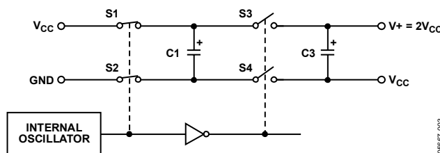
Figure 11. Charge Pump Voltage Double Operation
