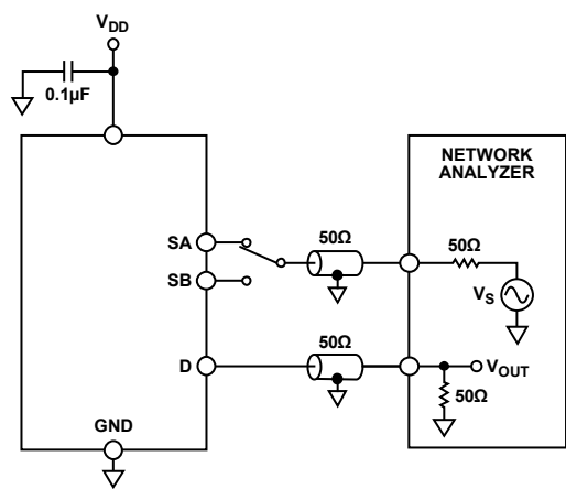
Figure 25. Bandwidth
