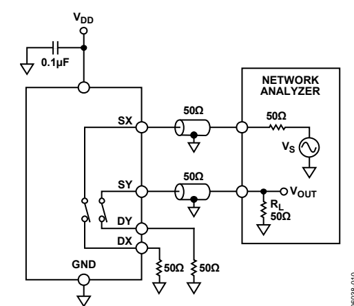
Figure 27. Channel-to-Channel Crosstalk
