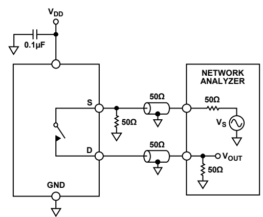
Figure 26. Off Isolation
