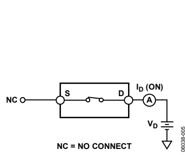
Figure 23. Off Leakage
