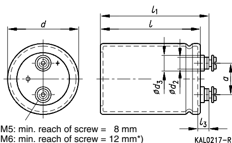
Type B43560 Ring clip/clamp mounting
