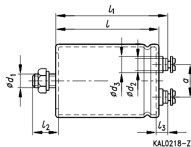
Type B43580 Threaded stud mounting
