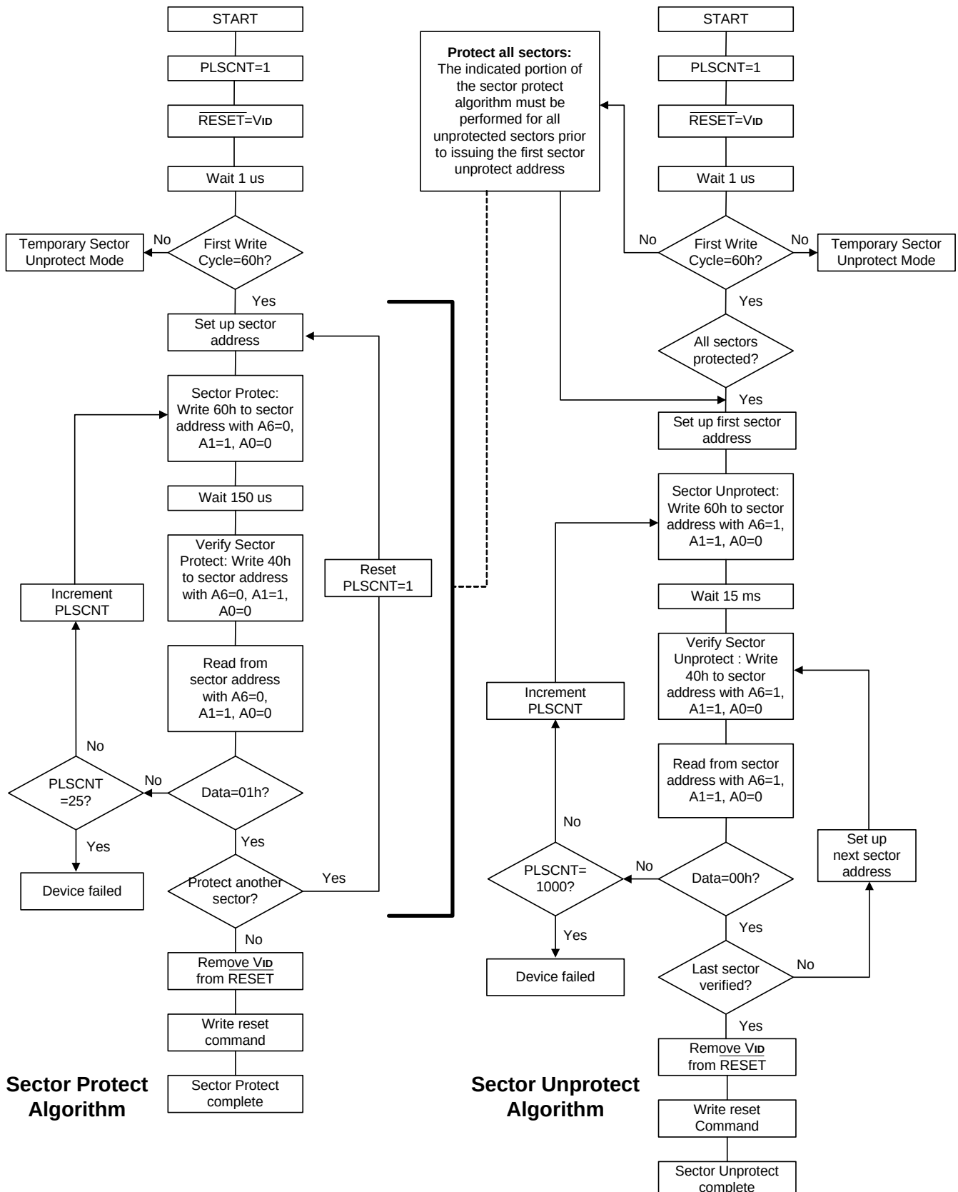
Figure 2-1. In-System Sector Protect/Unprotect Algorithms
