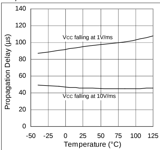
Figure 8. V_{CC} falling Propagation Delay vs. Temperature
