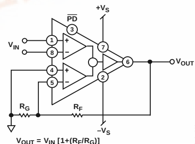
Figure 3. Typical Connection Configuration
