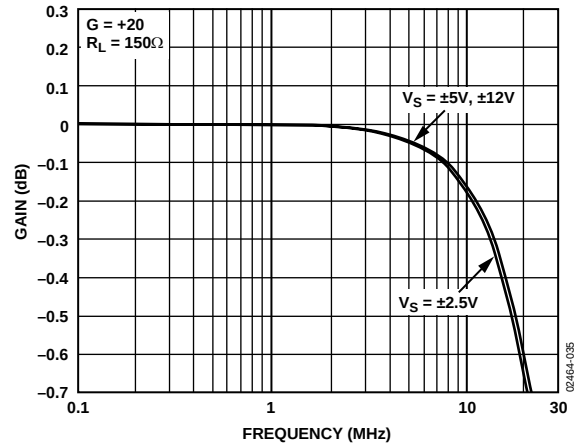
Figure 34. AD8129 Fine Scale Response vs. Supply
