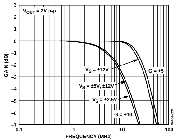
Figure 19. AD8130 Frequency Response vs. Supply, G = +5 , G = +10 , V_{OUT} = 2V p-p
