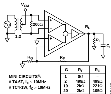
Figure 65. AD8129/AD8130 Basic Distortion Test Circuit, V_{CM} = 0V , Unless Otherwise Noted
