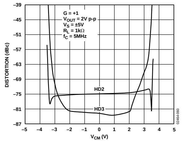
Figure 59. AD8130 Harmonic Distortion vs. Common-Mode Voltage
