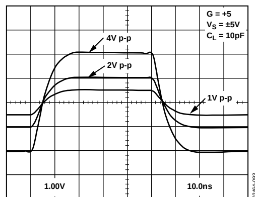
Figure 92. AD8130 Transient Response vs. Output Amplitude
