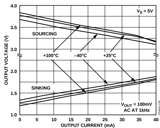
Figure 128. Output Voltage Range vs. Output Current, Typical 1% Gain Compression
