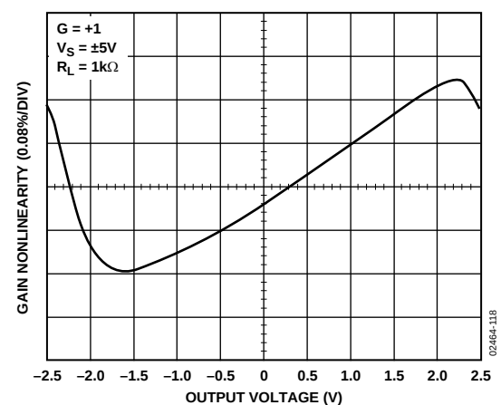
Figure 117. AD8130 Gain Nonlinearity, V_{OUT} = 5\text{ V p-p}
