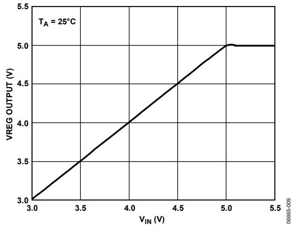
Figure 9. VREG in Dropout, No Load
