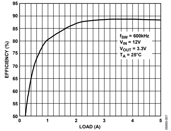
Figure 7. Efficiency vs. Load Current of Figure 54
