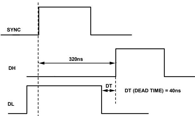
Figure 34. Synchronization
