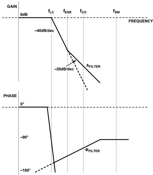
Figure 36. LC Filter Bode Plot
