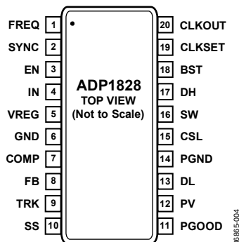
Figure 3. Pin Configuration
