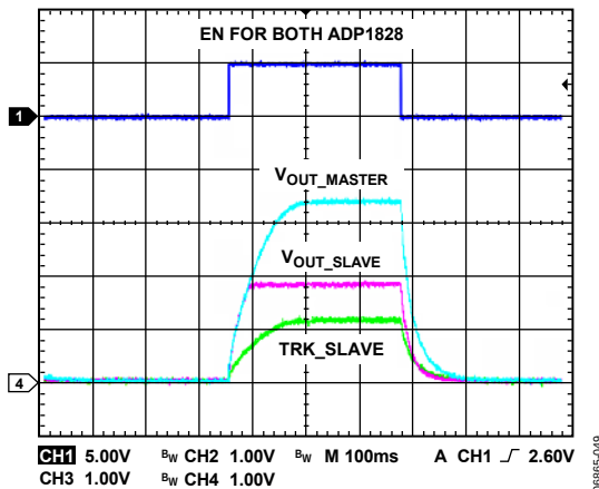
Figure 47. Ratiometric Tracking of Figure 46
