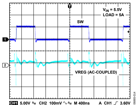
Figure 14. VREG Output of Figure 54
