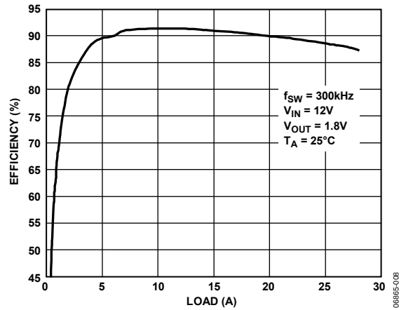
Figure 8. Efficiency vs. Load Current of Figure 56
