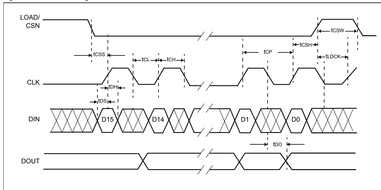
Figure 9. Interface Timing
