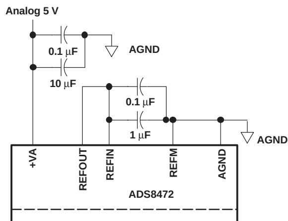
Figure 38. ADS8472 Using Internal Reference
