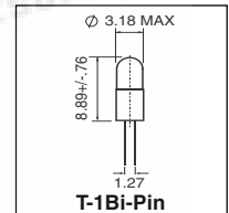
T-1 Bi-Pin
