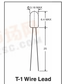
T-1 Wire Lead
