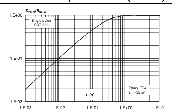
Figure 6. Relative variation of thermal impedance junction to ambient versus pulse duration (SOT-666)
