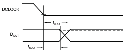
Voltage Waveforms for \text{D}_{\text{OUT}} Delay Times, t_{\text{DQ}}
