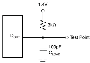
Load Circuit for t_{\text{DQ}} , t_r , and t_f
