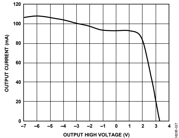
Figure 22. Output Current vs. Driver Output High Voltage
