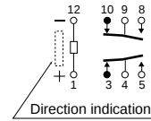
Schematic (Top view) Single side stable (Deenergized condition)
