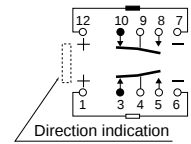
2 coil latching (Reset condition)
