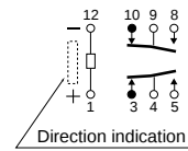
Schematic (Top view) Single side stable (Deenergized condition) 1 coil latching (Reset condition)
