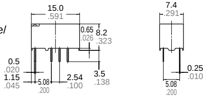
Single side stable/ 1 coil latching
