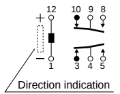
Schematic (Top view) Single side stable (Deenergized condition) 1 coil latching (Reset condition)
