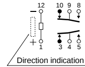
Schematic (Top view) Single side stable (Deenergized condition)
