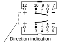
2 coil latching (Reset condition)
