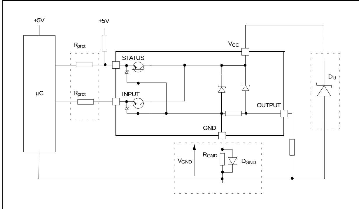
Figure 8. Application Schematic
