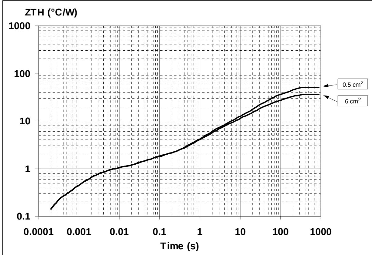
Figure 39. P 2 PAK Thermal Impedance Junction Ambient Single Pulse
