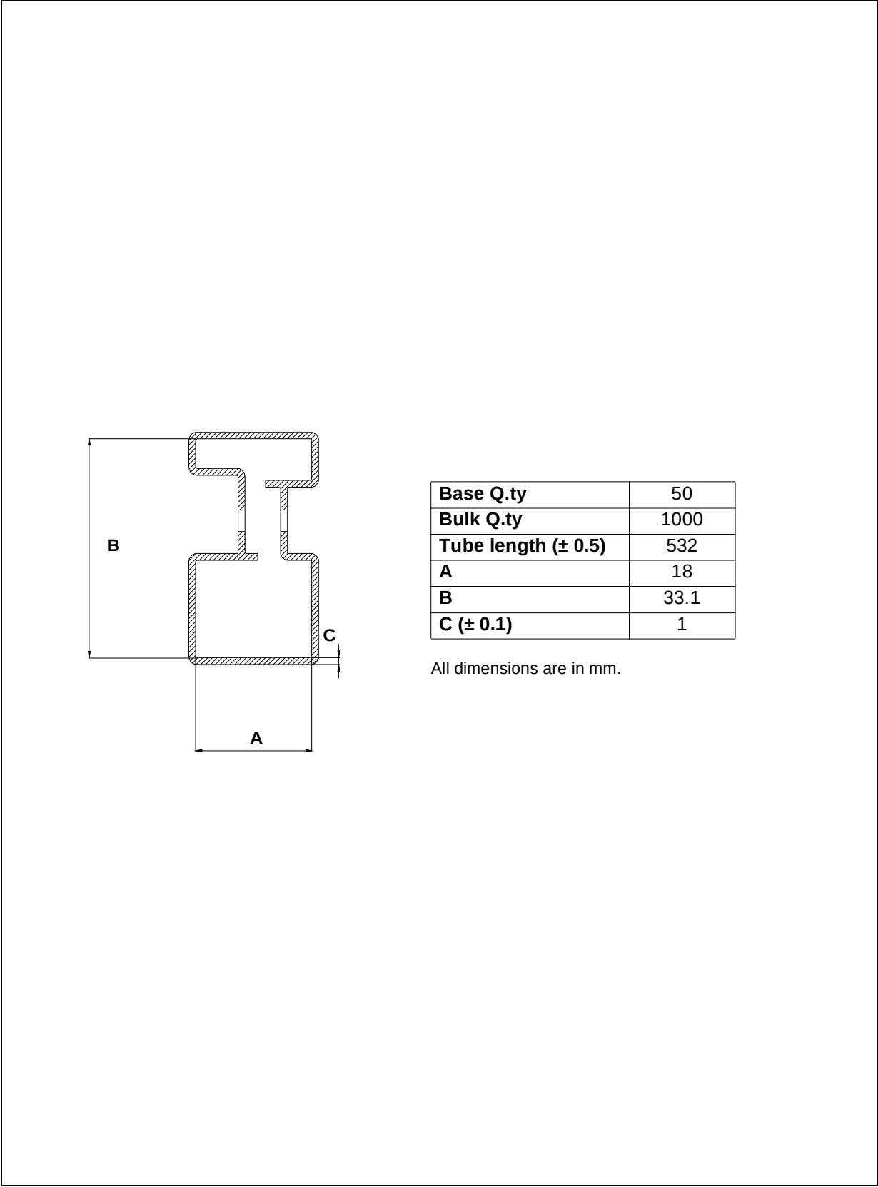
Figure 47. PENTAWAT TUBE SHIPMENT (no suffix)
