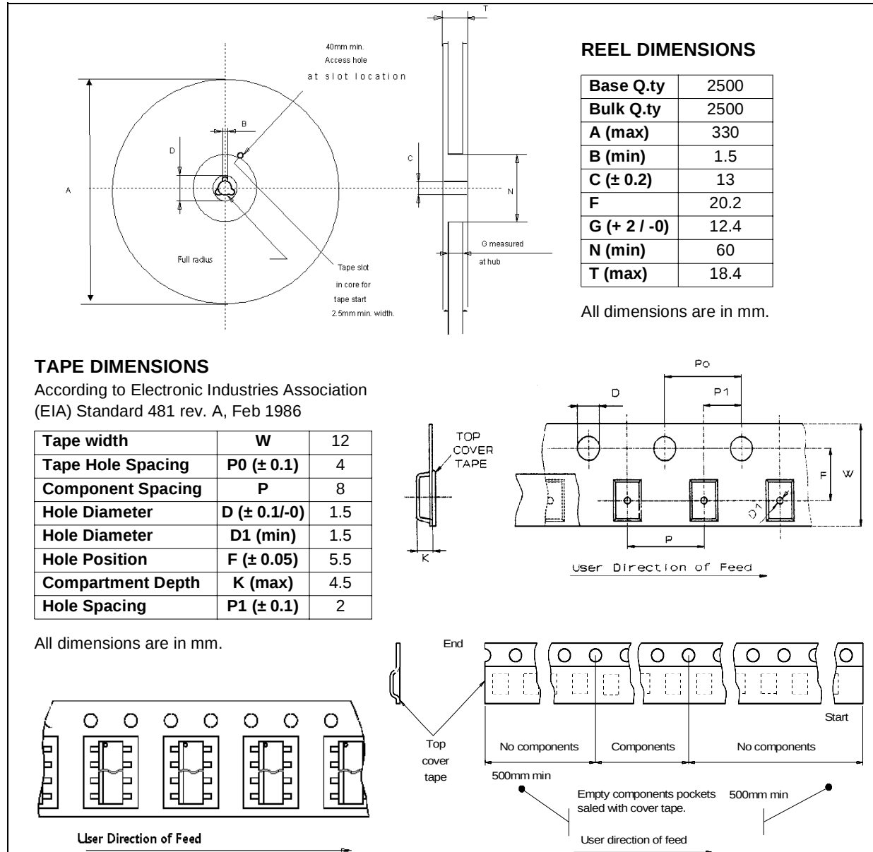
Figure 46. SO-8 TAPE AND REEL SHIPMENT (suffix "TR")
