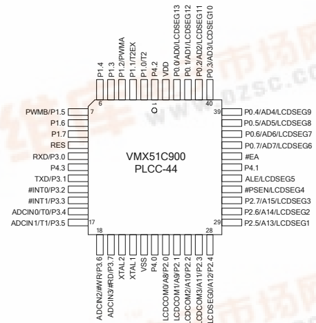
FIGURE 2: VMX51C900 PLCC-44 AND QFP-44 PIN OUT DIAGRAMS
