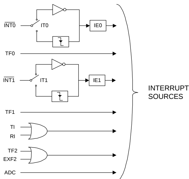
FIGURE 21: INTERRUPT SOURCES
