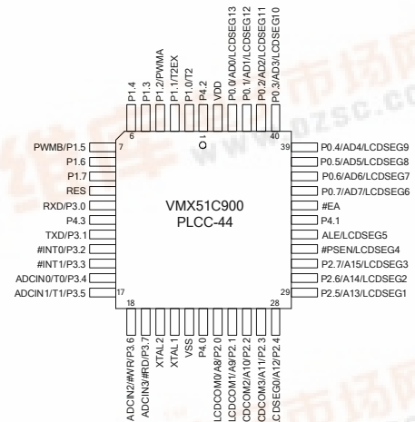
FIGURE 2: VMX51C900 PLCC-44 AND QFP-44 PIN OUT DIAGRAMS
