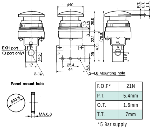
DIMENSIONS VM100 PUSH BUTTON-MUSHROOM
