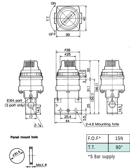
DIMENSIONS VM100 TWIST SELECTOR-2 POSITION
