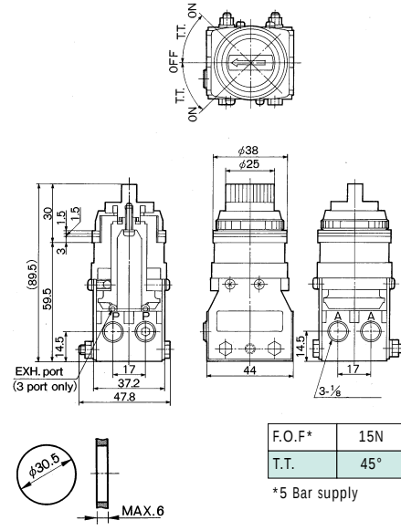
DIMENSIONS VM100 5/3 TWIST SELECTOR
