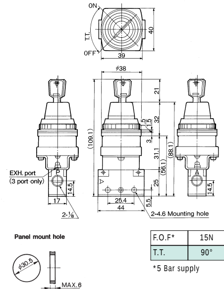
DIMENSIONS VM100 KEY SELECTOR-2 POSITION
