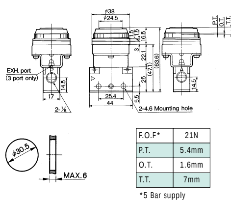
DIMENSIONS VM100 PUSH BUTTON-FLUSH
