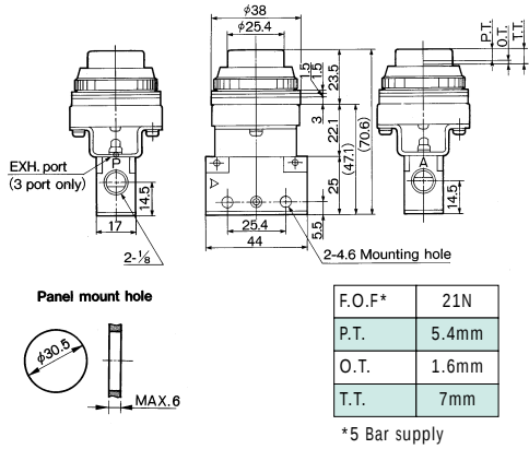
DIMENSIONS VM100 PUSH BUTTON-EXTENDED
