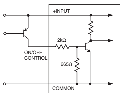
Figure 3. Driving the "Lucent Compatible" On/Off Control Pin
