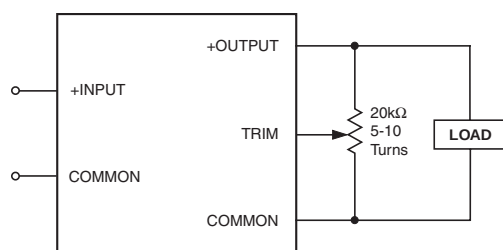
Figure 4. Trim Connections Using a Trimpot
