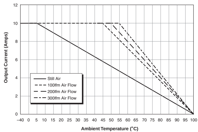
Temperature Derating for 10 Amp Models
