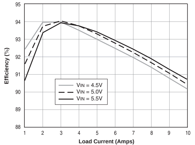
USN-3.3/10-D5 Efficiency vs. Line and Load
