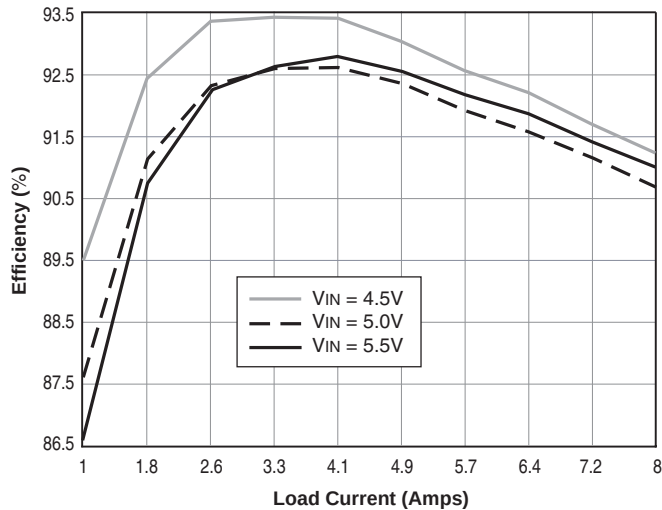
USN-3.3/8-D5 Efficiency vs. Line and Load
