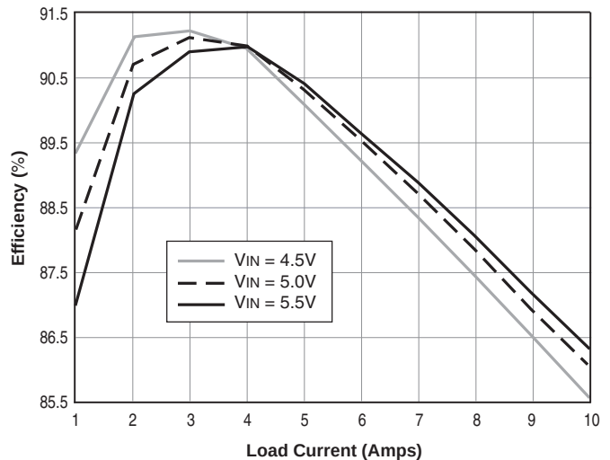
USN-1.8/10-D5 Efficiency vs. Line and Load
