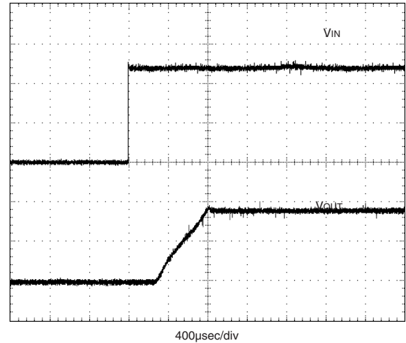
Typical Start-Up from VIN
