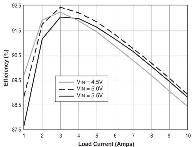
USN-2.5/10-D5 Efficiency vs. Line and Load
