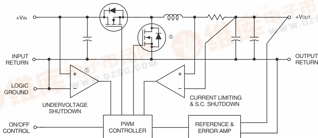
Figure 1. Simplified Schematic
