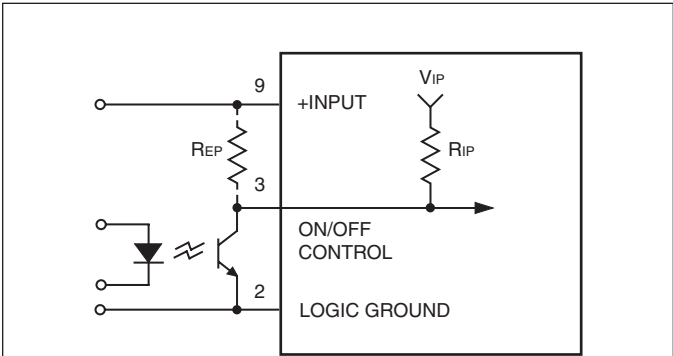
Figure 2. Driving the On/Off Control Pin
