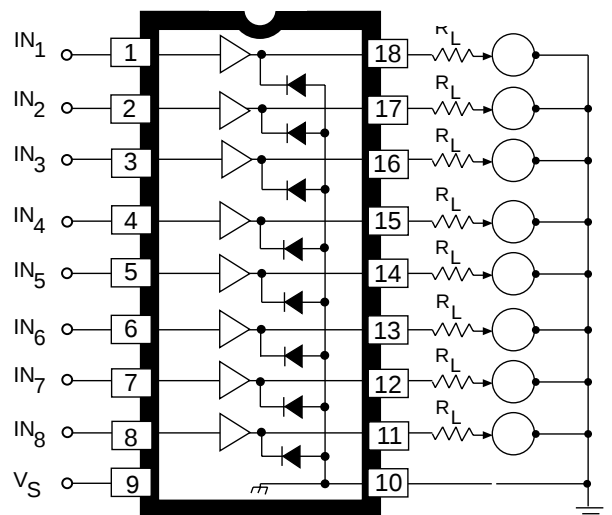
Typical electrosensitive printer application
