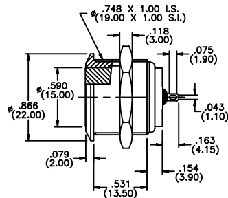
09 flat Act.& curved Bush.
