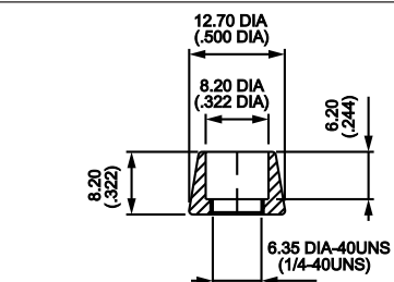
U1636 For caps U1140 & U2510
