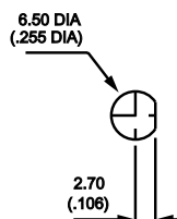
1/4" (6.35mm) flatted bush.
