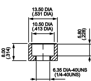
U840 For cap U480
