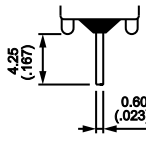
P0 Straight printed circuit
