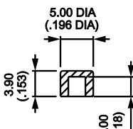
U4320 For 4 actuator only
