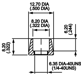
U1636 For cap U1140
