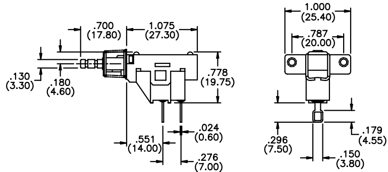
MECHANICAL OUTLINE
