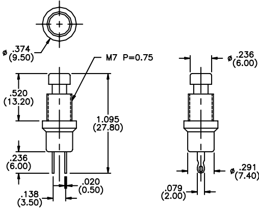
MECHANICAL OUTLINE
