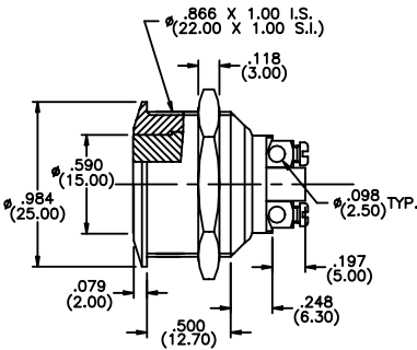
03 flat Act. & curved Bush.
