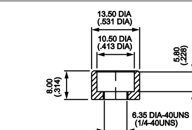
U840 For caps U480 & U2900
