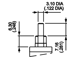
0000 Standard actuator w/smooth bushing
