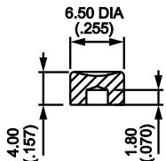
U570 Standard For standard actuator
