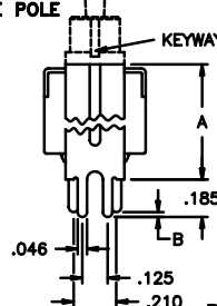
FRONT VIEW DOUBLE POLE
