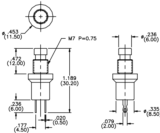
MECHANICAL OUTLINE
