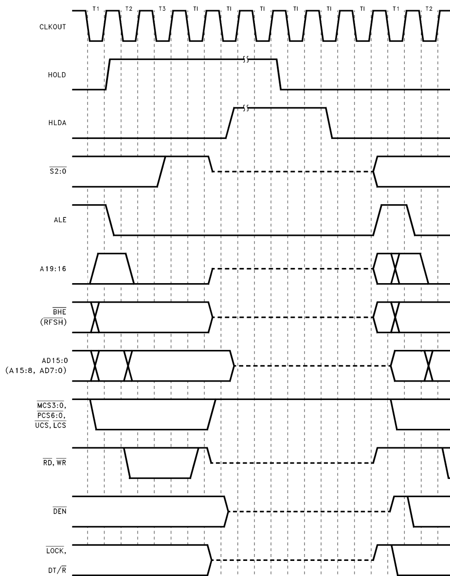
Figure 17. HOLD/HLDA Waveform
