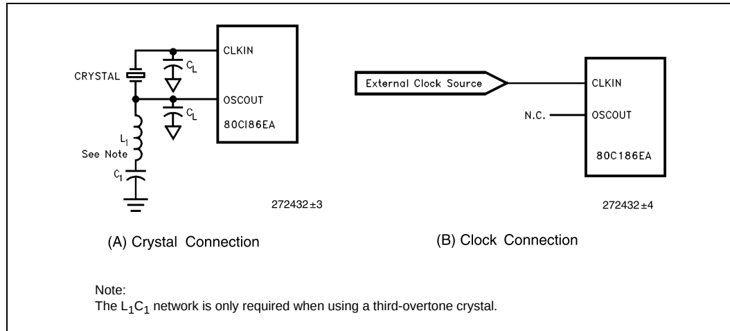
Figure 2. Clock Configurations
